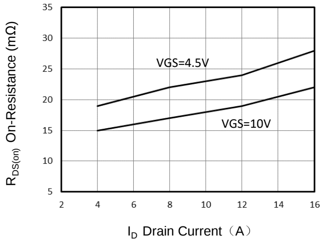
Figure 3. Drain-Source On-Resistance
